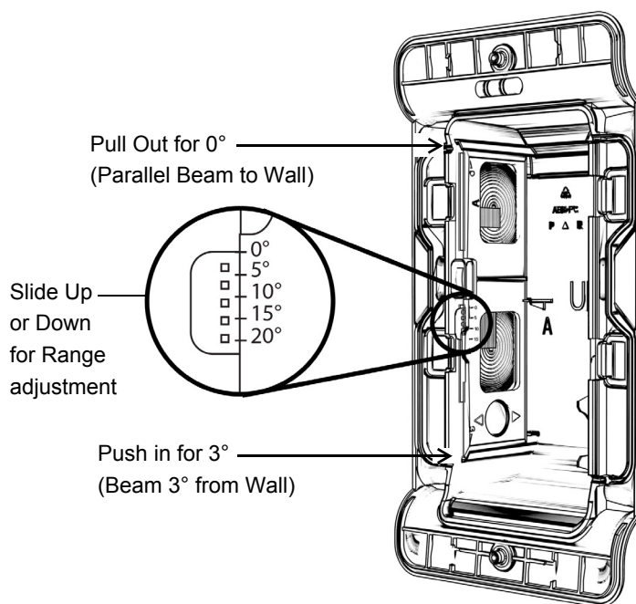
Figure 2 : Beam Adjustment
